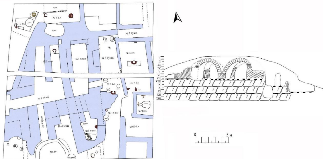
6-rasm. 2022 yilgi qazishmalar natijasida aniqlangan mudofaa inshootining rejasi va kesmasi
