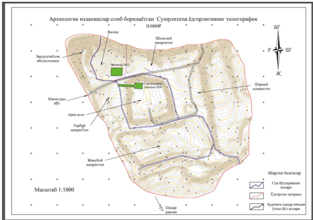
17-rasm. Suyurlitepa yodgorligining topografik rejasi.
